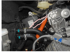
Turn the ignition switch OFF and disconnect the auxiliary 12V battery positive (+) connector (A).
