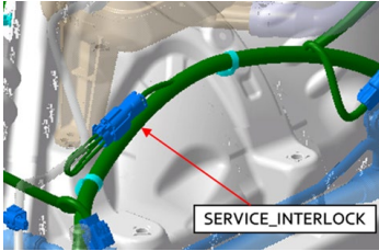
3. Disconnect service interlock connector
