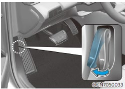
Pull the release lever to unlatch the hood. The hood should pop open slightly.
