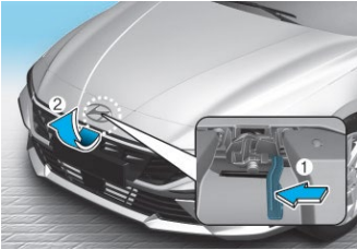
2. Raise the hood
