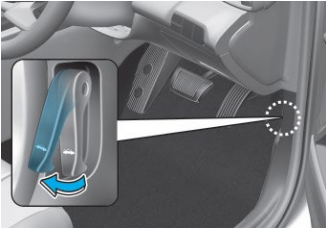
1. Pull the release lever
