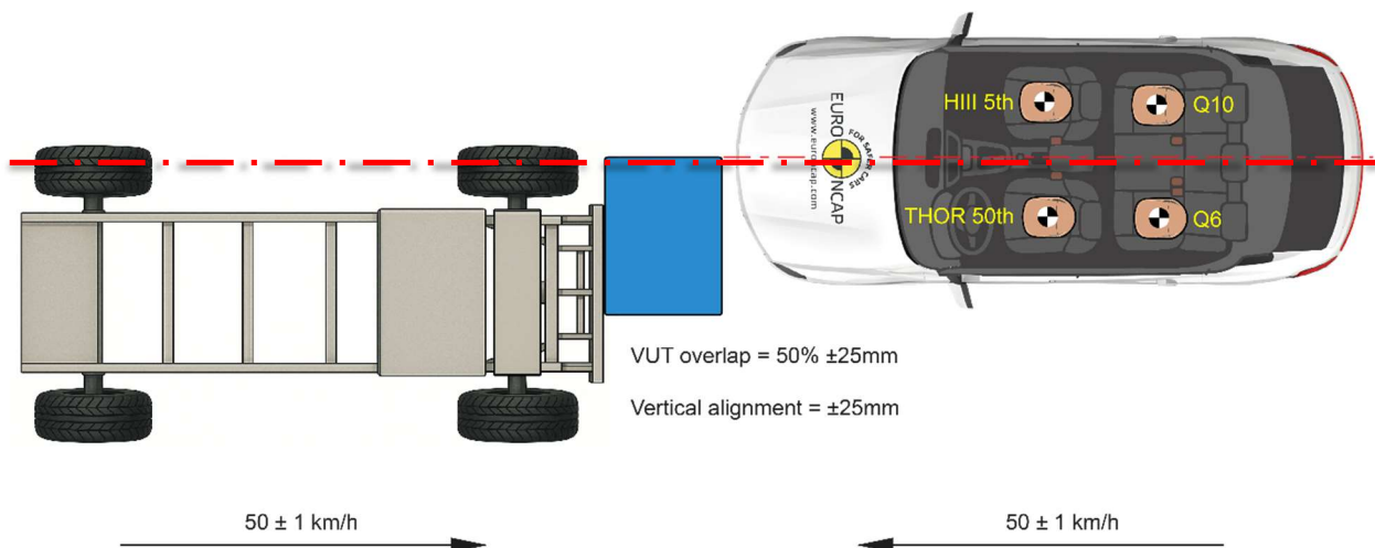
Figure 1 MPDB test
