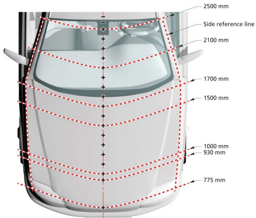
Figure 7: Headform test area
