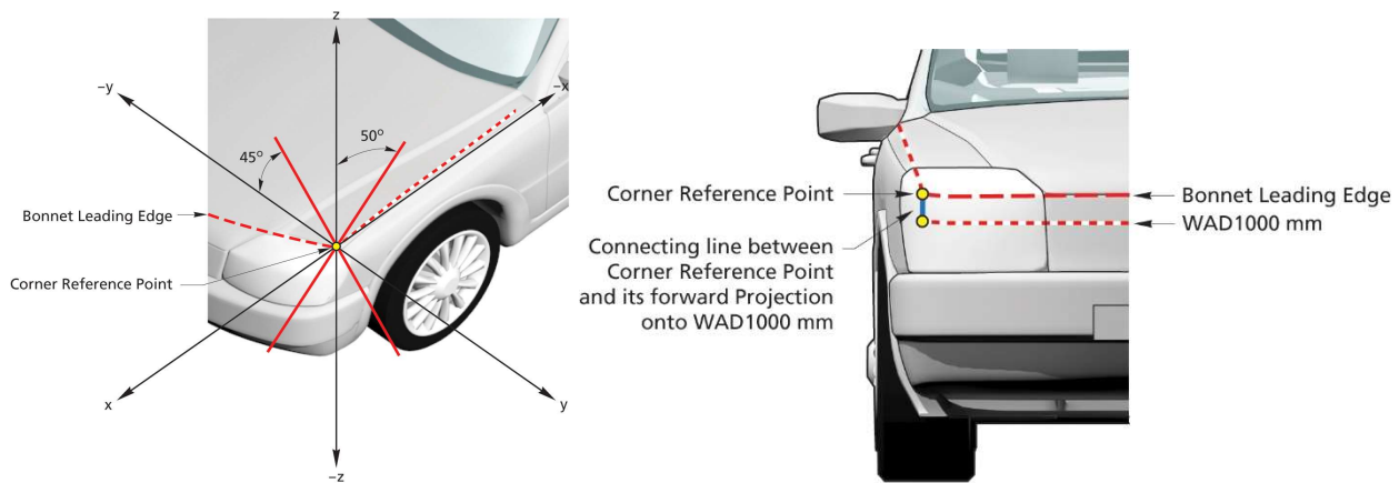
Figure 8: Determination of the corner reference point
