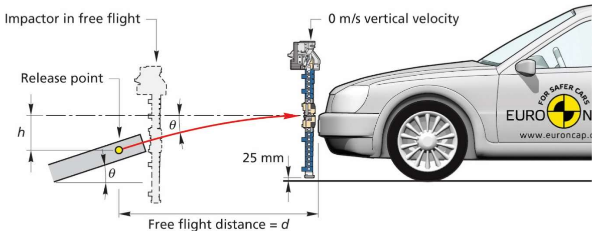
Figure 31 Ballistic compensation
