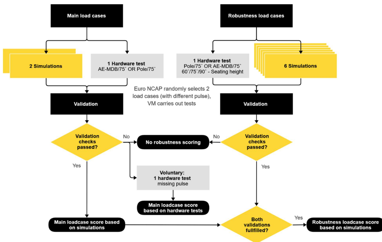
Figure 4: Far side impact
