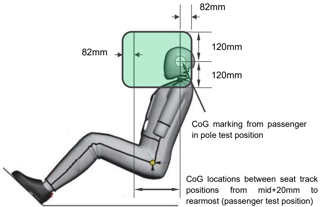
Figure 12: Far side protection zone
