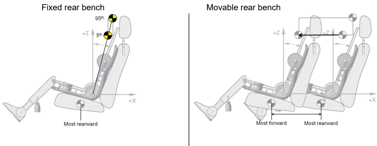
Figure 9: HPD zone rear seat row(s)
